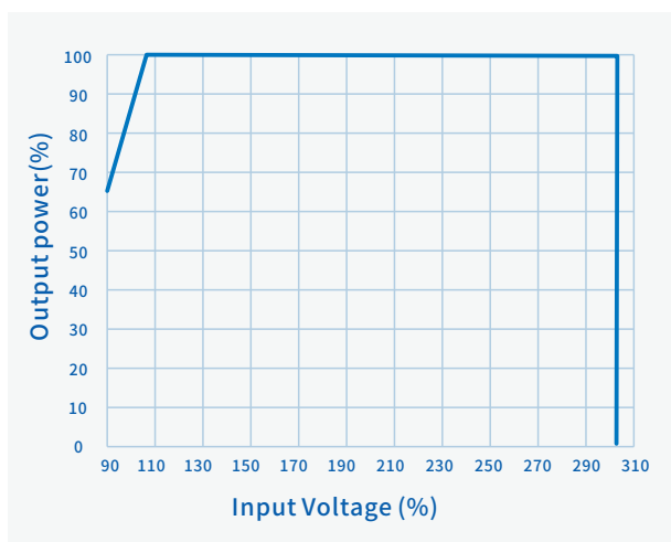
O/P Power Vs. Input Voltage (Automatic Derating)
