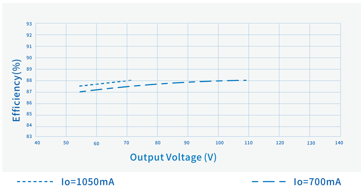
Efficiency Vs. Output Voltage (Vin=120Vac)
